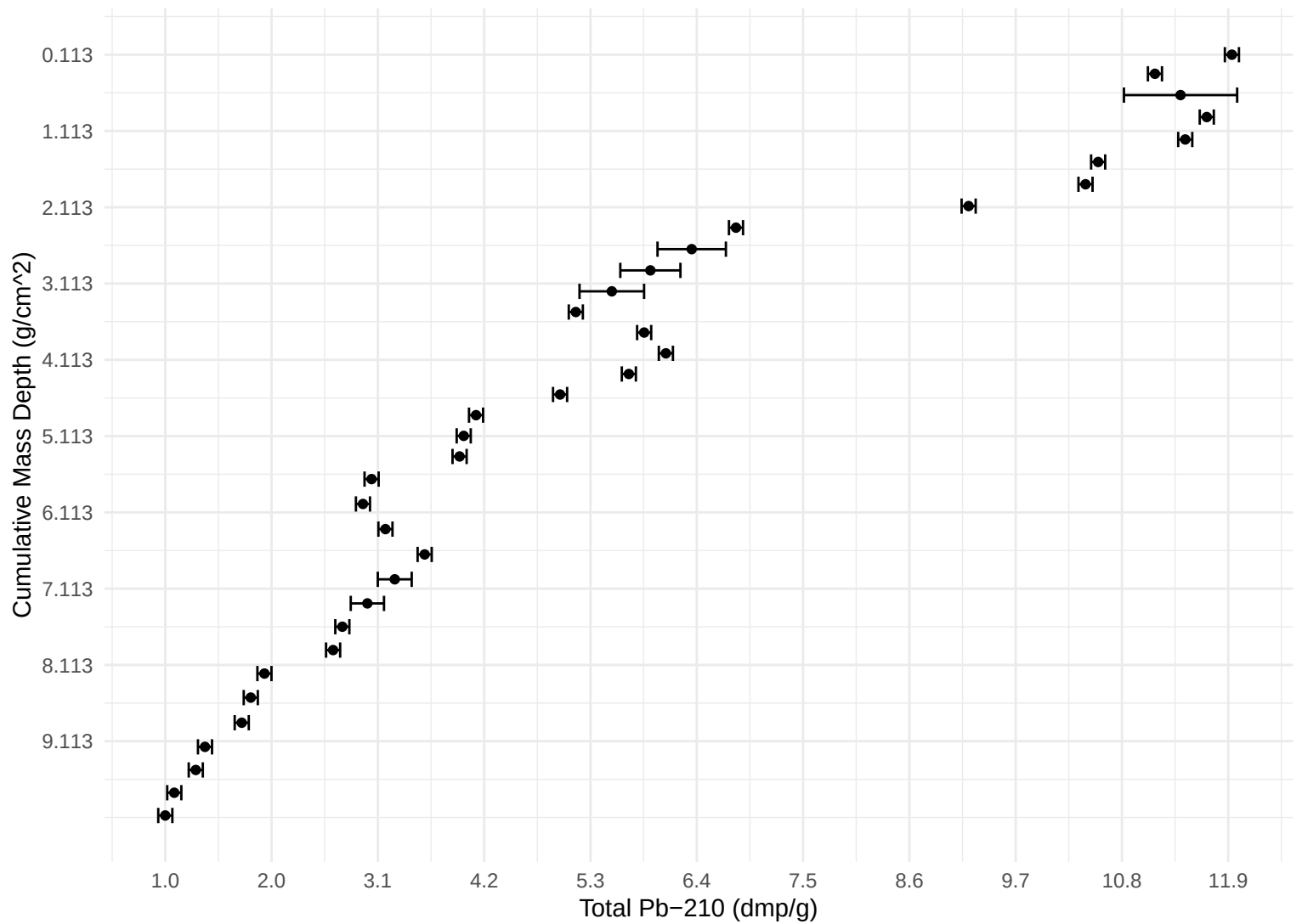
Total Pb-210 vs Cumulative Mass Depth
